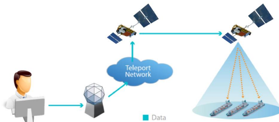
Figure 2 – Basic concept of the Iridium Global Satellite EGC-SafetyCast service
