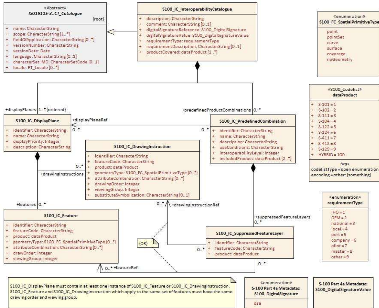
Figure 4.3 - Basic interoperability catalogue (Levels 1 and 2)
