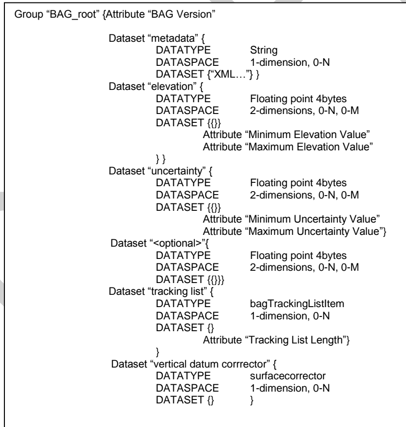
Fig A1 - Structure of BAG Data Encoding using HDF5
