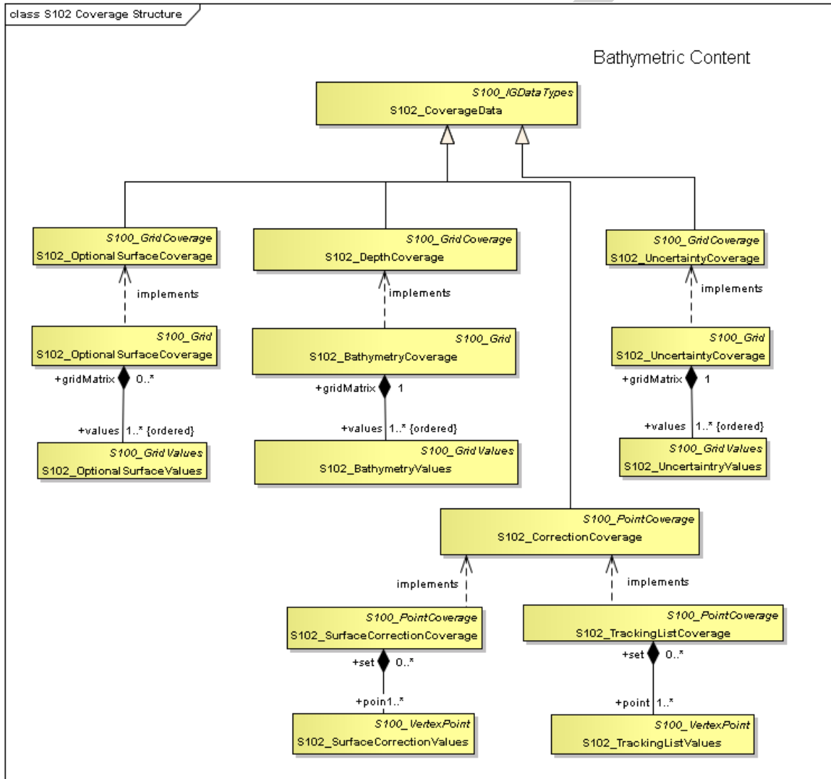
Fig 3 – Coverage Structure of S-102
