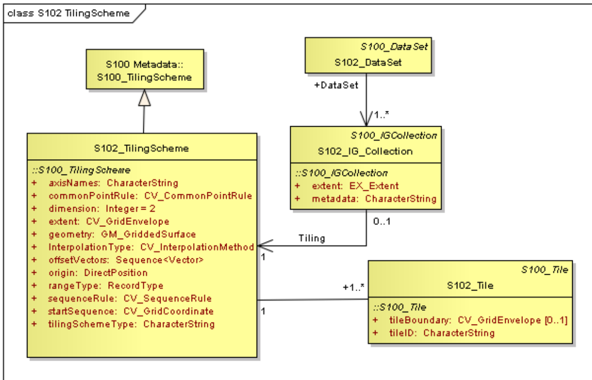
Fig 8 - S-102 Tiling Scheme
