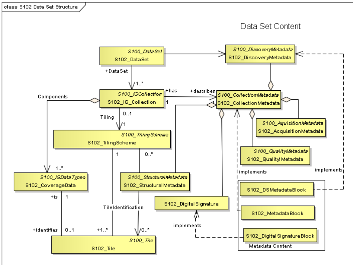
Fig 2 – Data Set Structure of S-102
