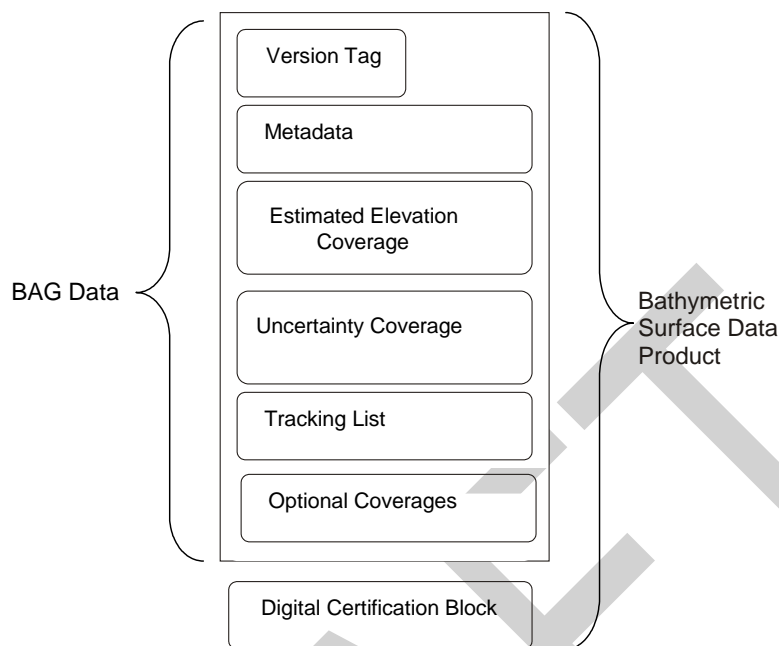
Fig 1 - Overview Structure of S-102
