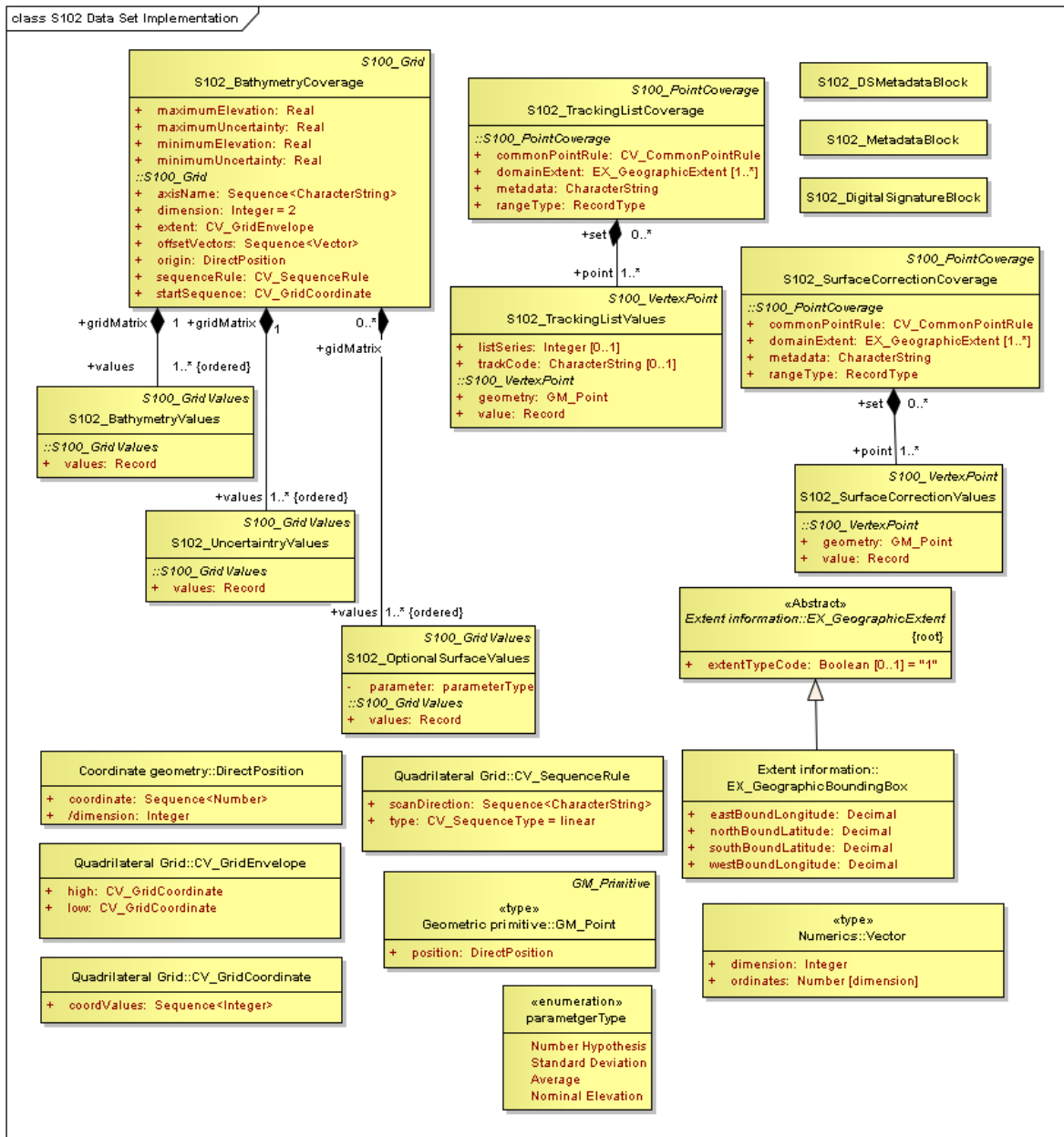
Fig 4 - Implementation Classes of S-102
