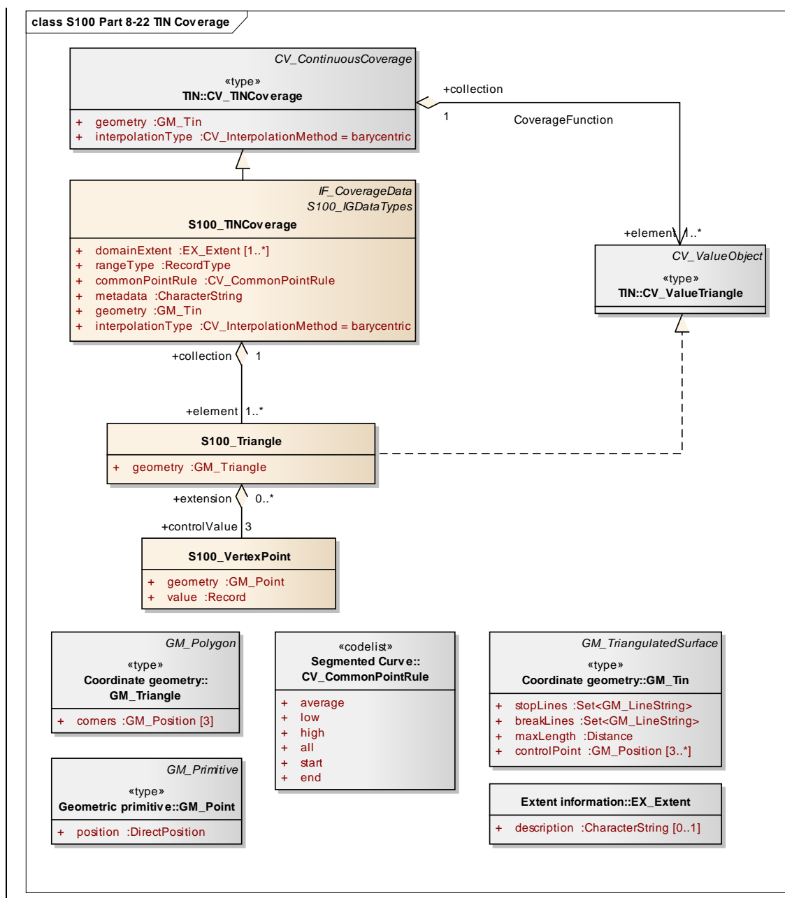
Figure 8-22 - S100_TIN Coverage
