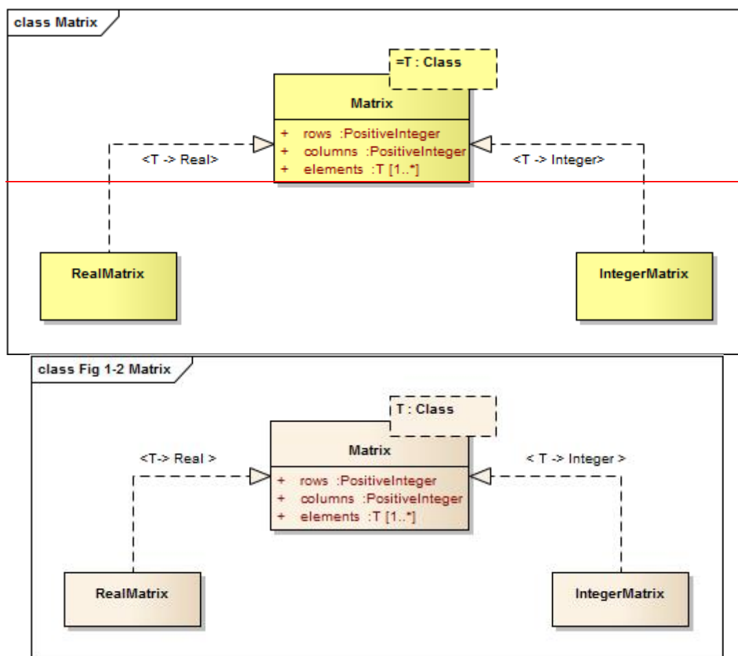
Figure 1-2 – Matrix
