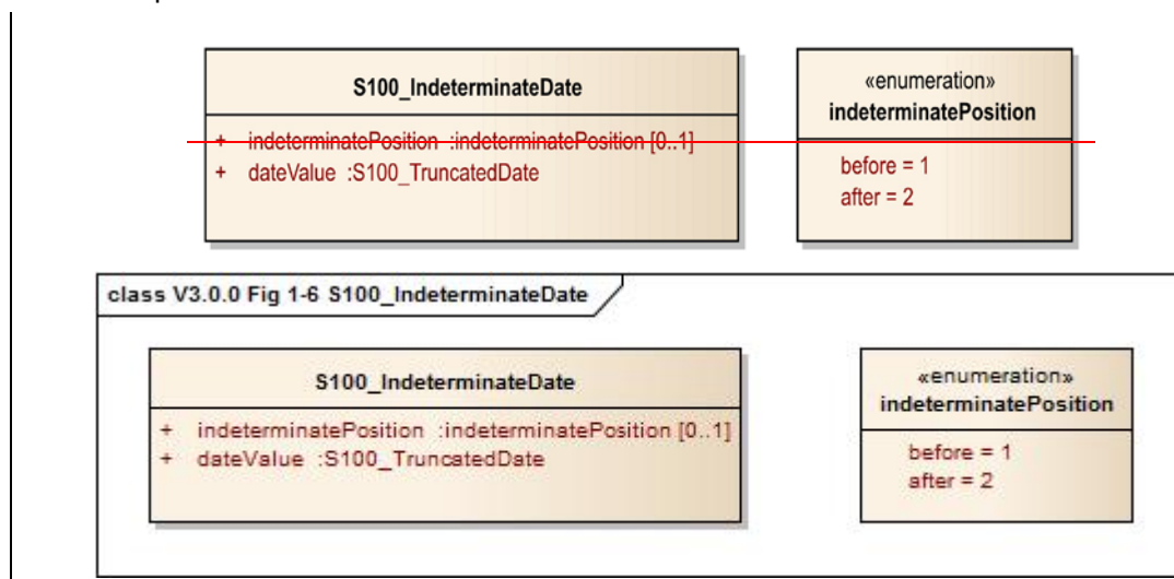
Figure 1-6 – S100_IndeterminateDate
