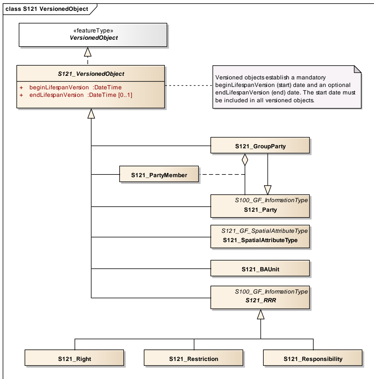
Figure 11- Versioned Objects
