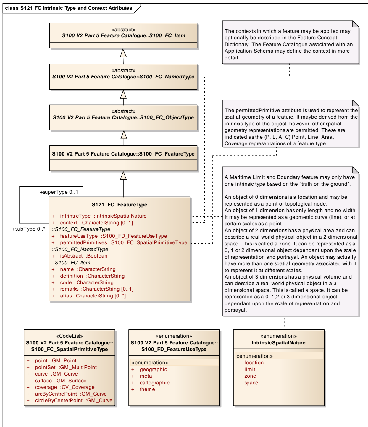
Figure 8 – S-121 Feature Concept Dictionary Entries with Intrinsic Type
