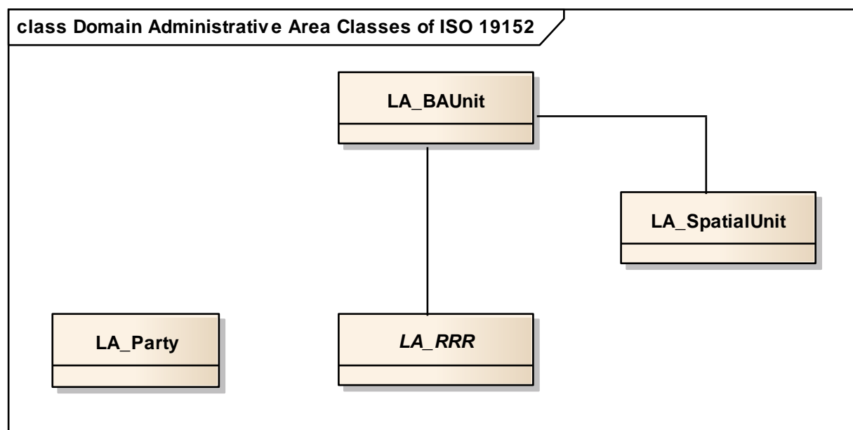
Figure 9- Domain Administrative classes
