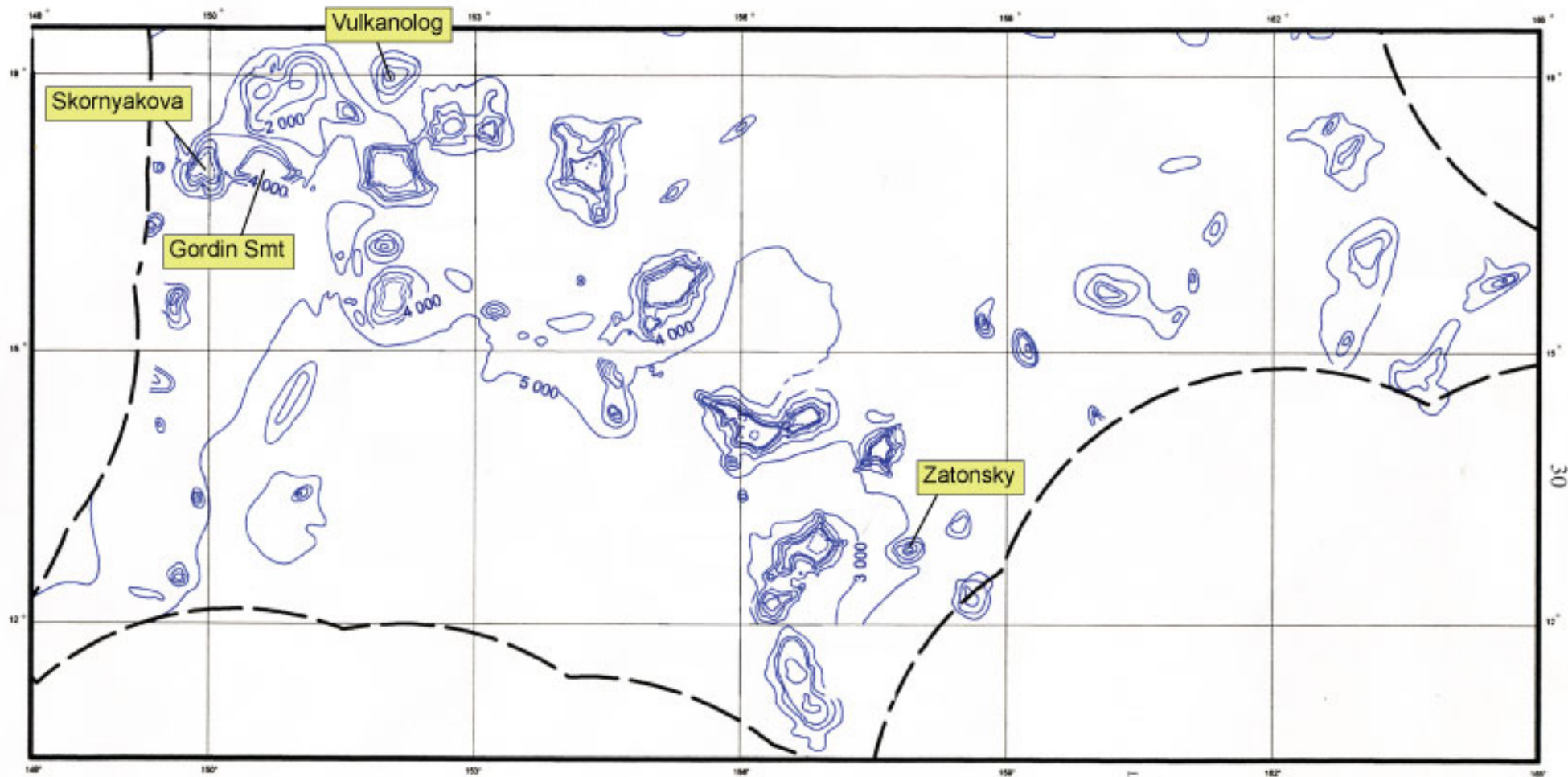
Bathymetry diagram of Magellan seamounts
