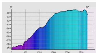
Fig.4. Profile across Gungpa Hills
