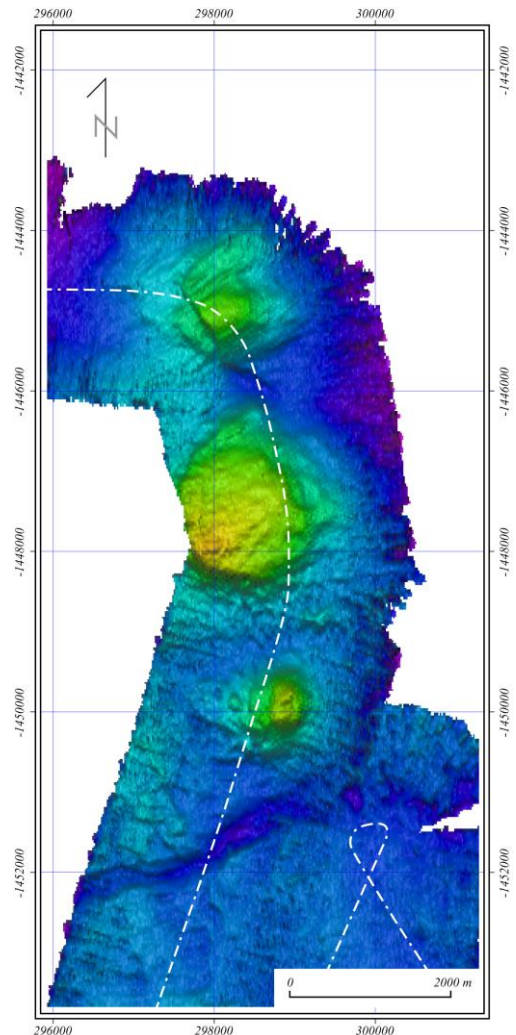
Fig.2. The track lines in Survey area
