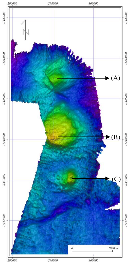
Fig.1. 2-D Bathymetric Contour map of the Gungpa Hills
