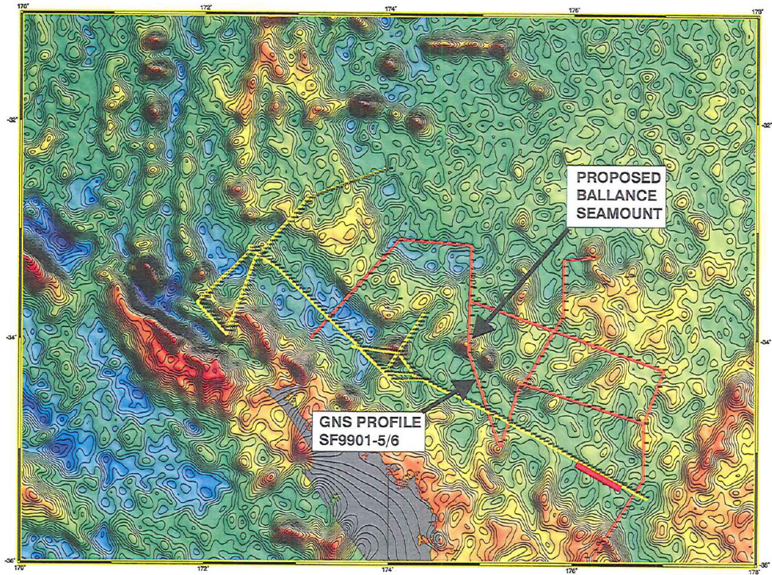
SATELLITE GRAVITY MAP
