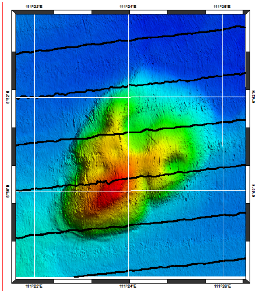
Track lines for Rentap Hill
