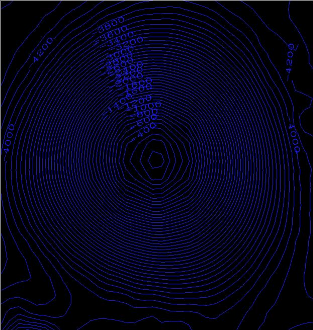
Chac Seamount - Depth in meters
