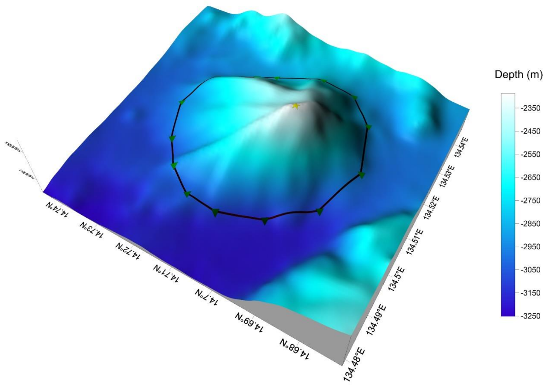
Fig.4 3-D topography map of Chunfen Hill
