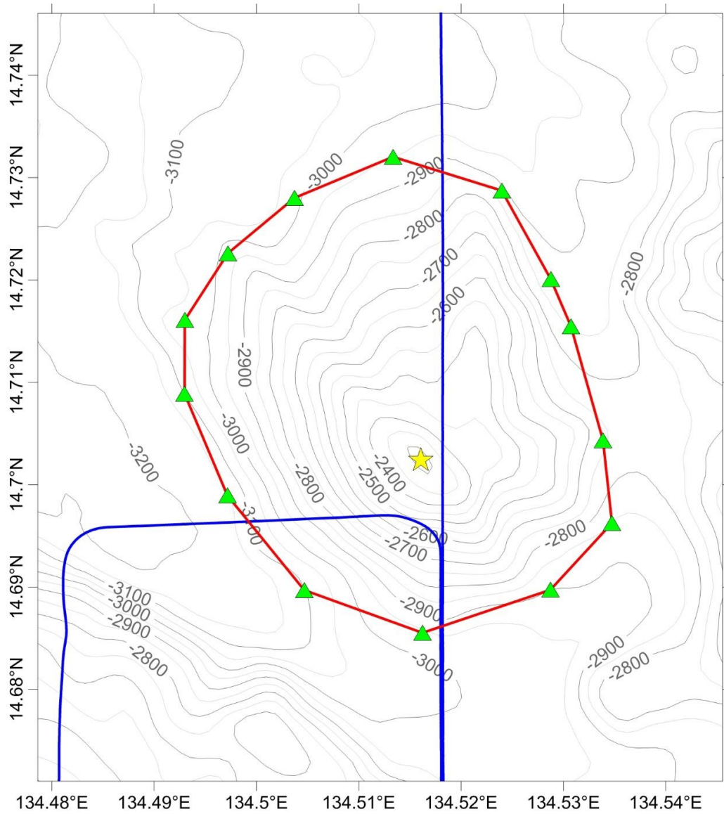
Fig.3 Bathymetric map of Chunfen Hill, showing track lines (Contours are in 100 m, blue lines are survey lines)
