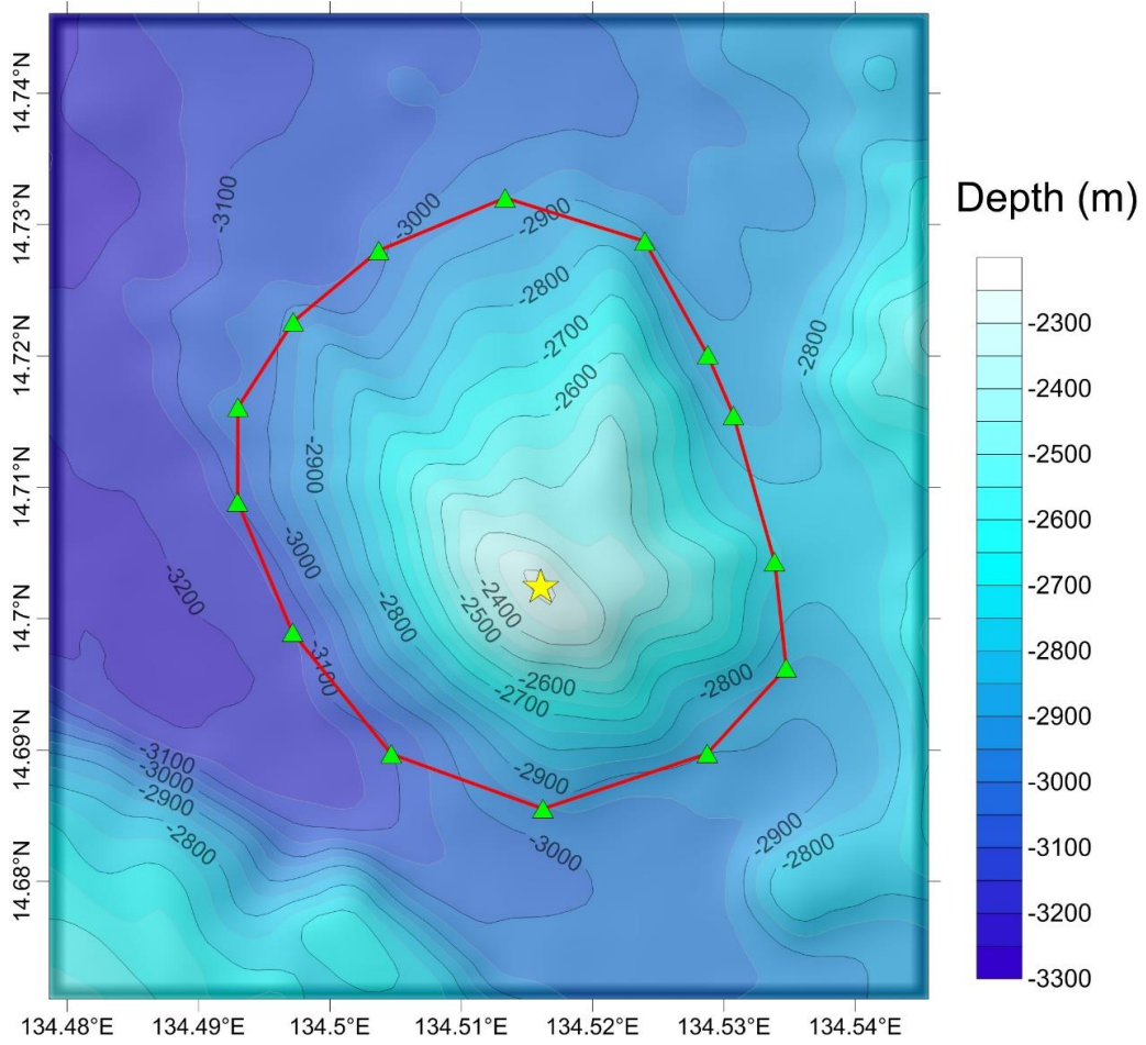
Fig.2 Bathymetric map of Chunfen Hill (Contours are in 100 m)
