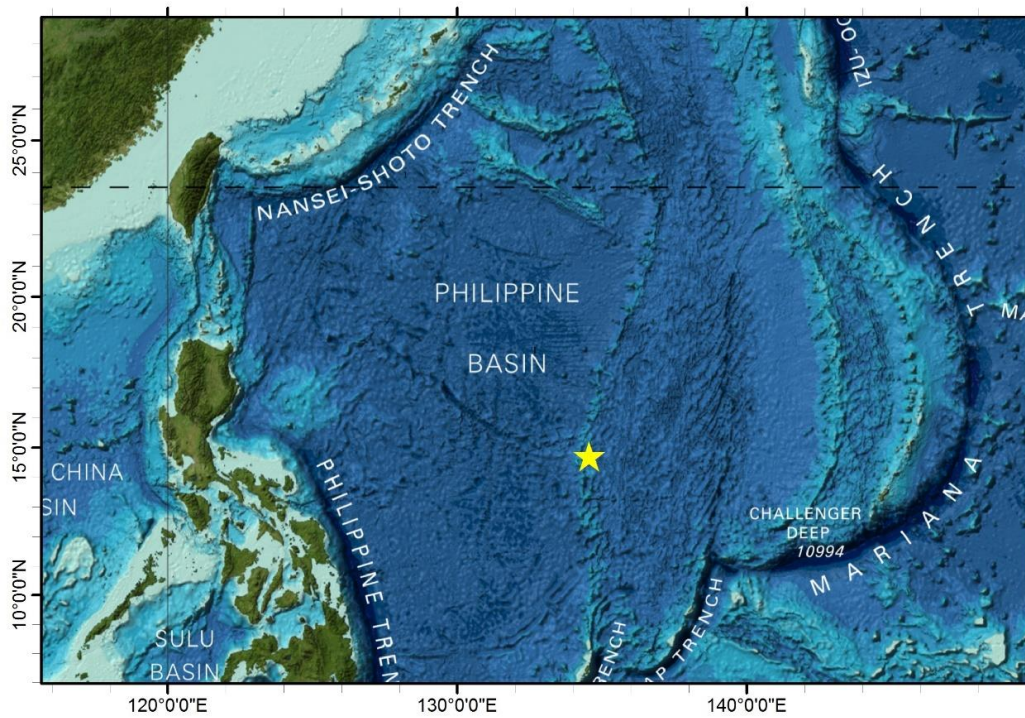
Fig.1 Index map showing the location of Chunfen Hill
