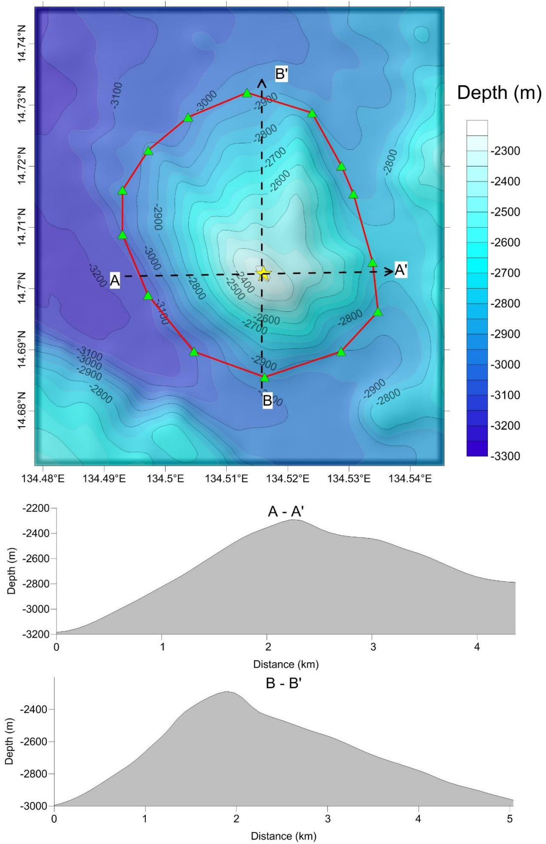
Fig.5 Bathymetric map and profiles of Chunfen Hill
