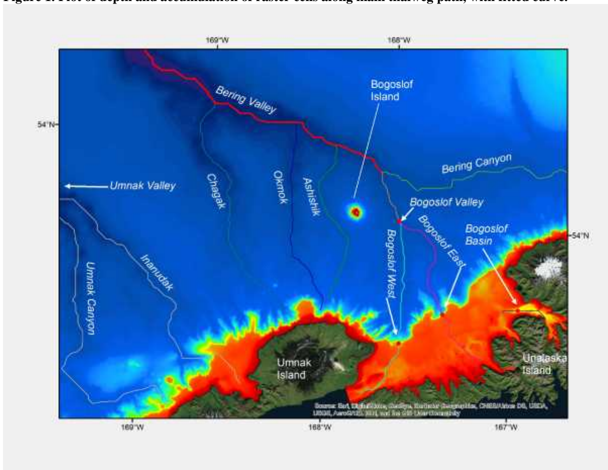
Figure 2. Modified version of Fig 7. (Zimmermann & Prescott, 2018) “Thalwegs of the Bering Canyon area of the eastern Bering Sea slope” showing proposed Bogoslof Canyon West place name.
