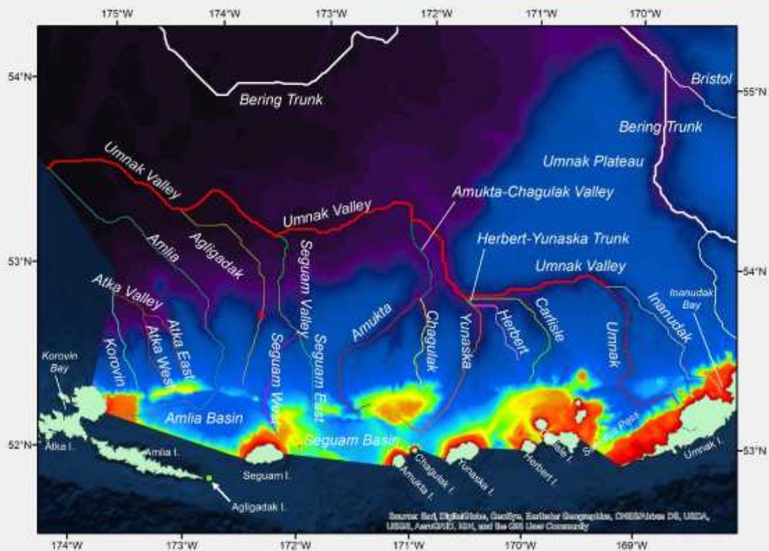
Figure 2. Modified version of Fig 6. (Zimmermann & Prescott, 2018) "Thalwegs of the Umnak Canyon area of the eastern Bering Sea slope" showing proposed location for Agligadak Canyon place name.
