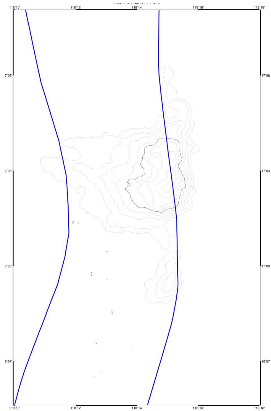
Figure 3. Bathymetric map of Dalos Hill showing track lines.
