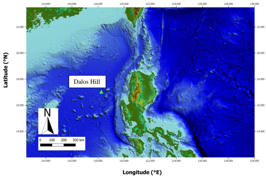
Figure 1. Index map showing the location of Dalos Hill.
